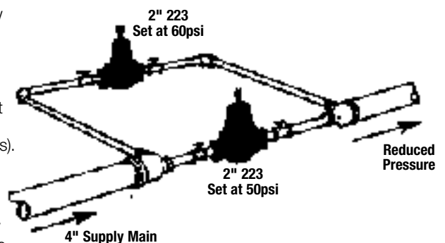
Fig. 4 – Parallel Installation
