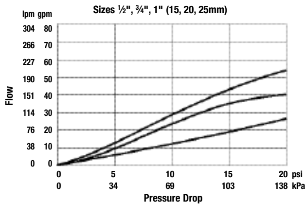
Chart No. 3 – Series 223
