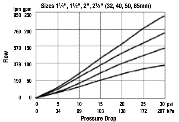
Chart No. 3A – Series 223
