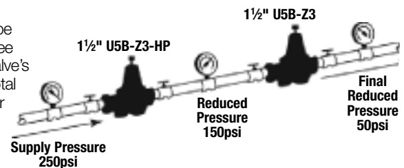
Fig. 3 – Two-stage serial reduction configuration
