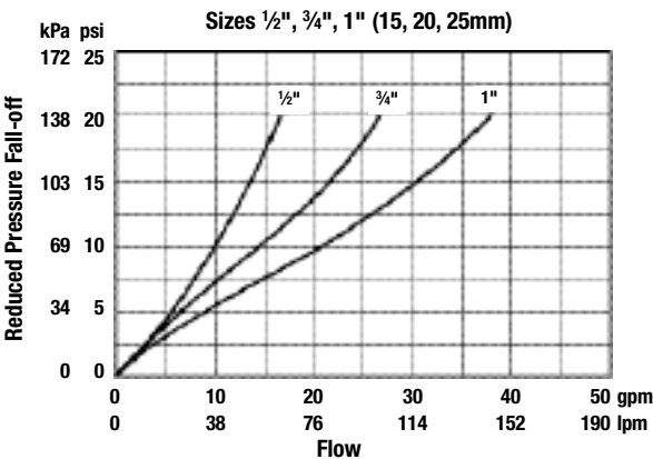
Chart No. 1 – Series U5B-Z3
