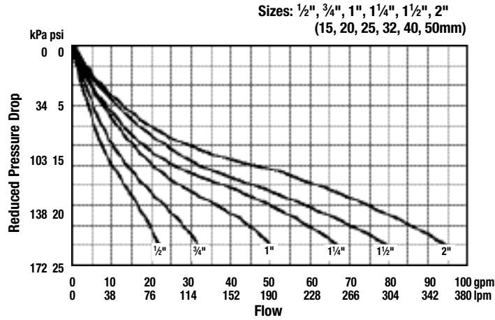
Chart No. 2 – Series 25AUB-Z3
