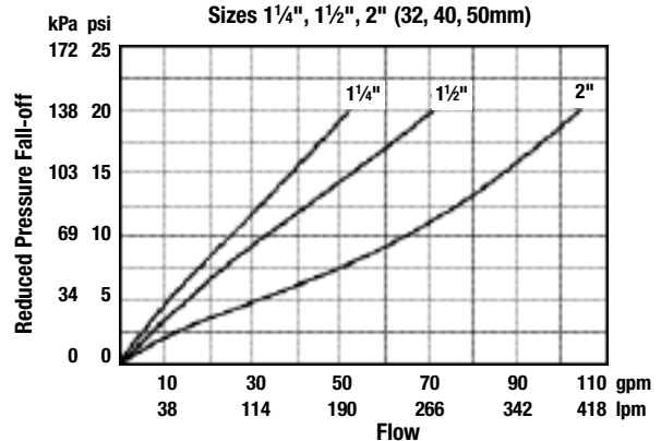
Chart No. 1A – Series U5B-Z3
