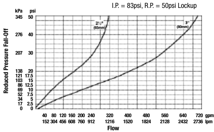
Chart No. 2A – Series N223B
