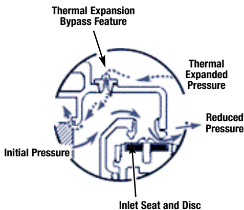
Fig. 2 – Watts Thermal Expansion Bypass feature
